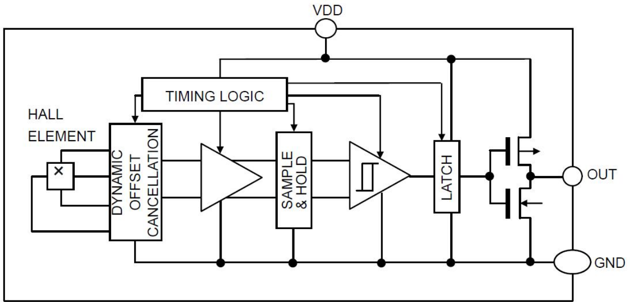
Figure 3, Block Diagram of AS1890
